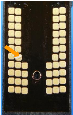
Figure 9 - Interconnect pad with debris (arrow)
