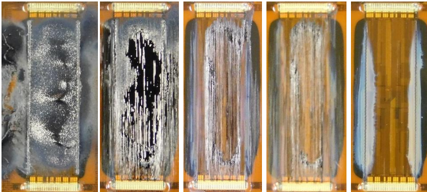
Figure 7 – The photo on the left shows the printhead before wiping, the middle photos show the printhead after successive dry wipes, and the photo on the right shows the printhead after a wipe with deionized water
