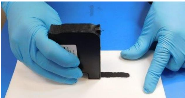
Figure 5 – “Wicking wipe” technique for removing hardened deposits of ink and debris (later wipe)
