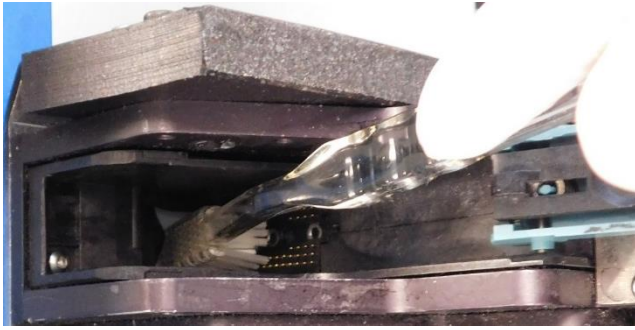
Figure 11 – Example of using a toothbrush to clean the pen pocket
